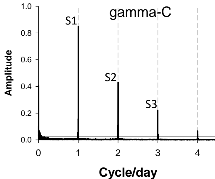
Figure 6: Spectra (FFT) of measurements of g-C. The confidence level (99.9%) is also shown. (A 99.9% critical limit is that level where in only 1 of 1000 separate random noise sets would the largest peak attain this height.)
