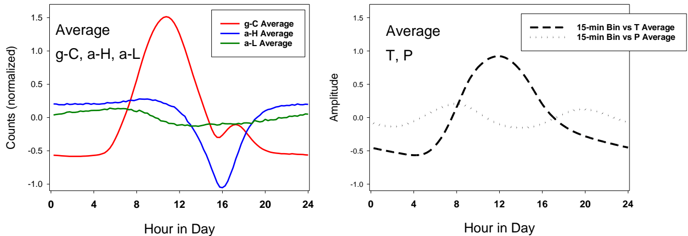
Figure 5: Comparison using the same normalized scale of variation of the daily variation of averages at the nuclear detectors (left), and ambient temperature and barometric pressure (right).
